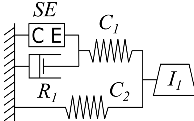
Fig. 4.12: The Hill model with five basic elements: contractile element, CE ; damping element, R_1 ; series elastic element, C_1 ; parallel elastic element, C_2 ; and inertial element, I_1 .
