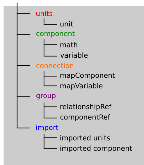
Fig. 3.9: Key entities in a CellML model.
