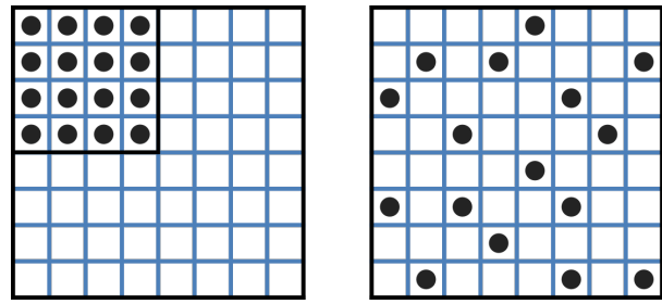
Fig. 3.1: Distribution of microstates in a system [J97]. The 16 particles in a confined region (left) have only one possible arrangement ( W = 1 ) and therefore zero entropy ( k_B \ln W = 0 ). When the barrier is removed and the number of possible locations for each particle increases 4x (right), the number of possible arrangements for the 16 particles increases by 416 and the increase in entropy is therefore \ln(416) or 16 \ln 4 . The thermal energy (temperature) of the previously confined particles on the left has been redistributed in space to achieve a more probable (higher entropy) state. If we now added more particles to the container on the right, the concentration would increase and the entropy would decrease.
