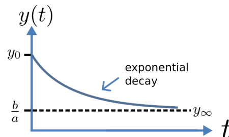
Fig. 6.4: Solution of 1 st order equation.
